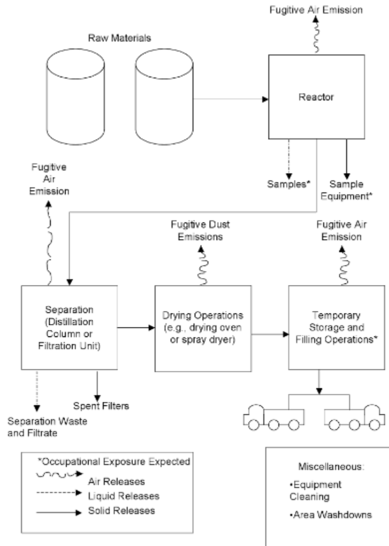
Generic Chemical Manufacturing Process Flow Diagram
